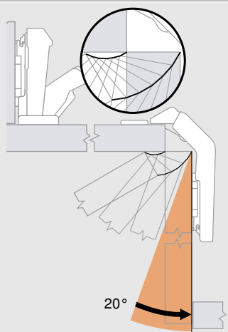
CLIP top 60° Bi-Fold Hinge
